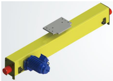
For single girder crane
