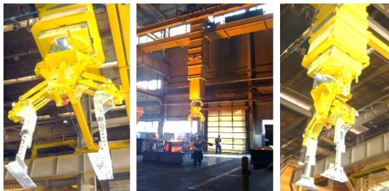
Clamp with Telescopic sleeve
